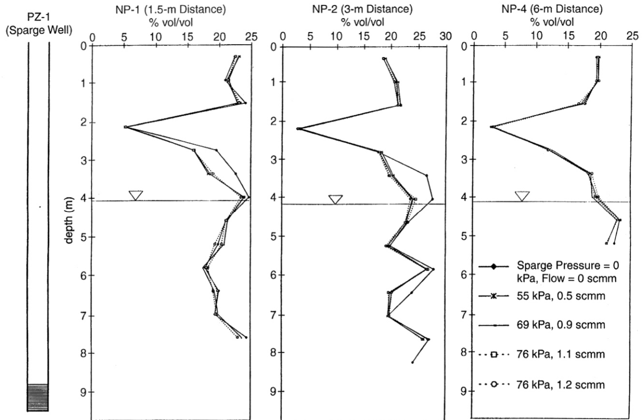
Figure 4-6. Moisture profiles obtained by neutron logging at 1.5, 3, and 6 m from the IAS well during various stages of the IAS test, showing the pre-test water table elevation for reference. Differences between the baseline measurement (sparge pressure = 0, flow = 0) and all subsequent measurements indicated the minimal air saturation due to IAS at this highly stratified site (after Baker et al. 1996).
