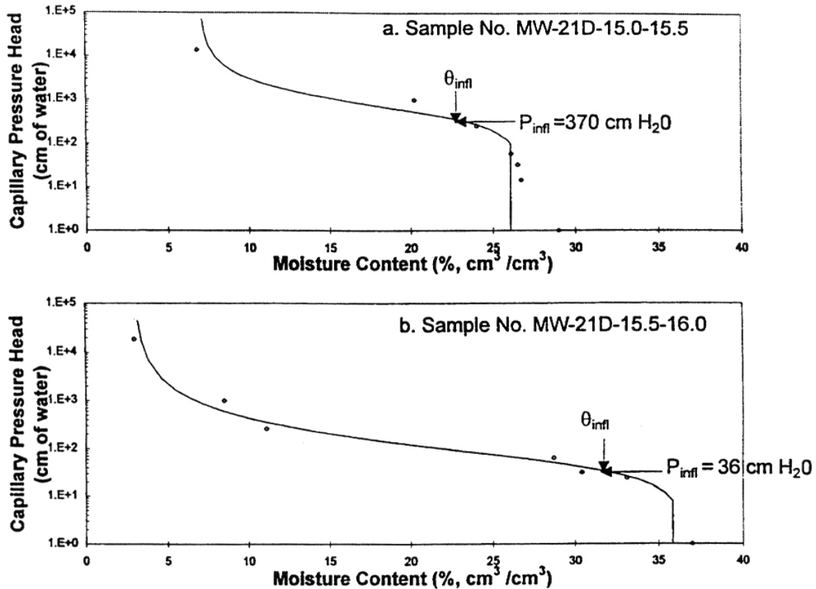
Figure 3-2. Capillary pressure head vs. moisture content for two adjacent soil horizons. Intact cores collected from adjacent soil layers within the sparge zone were submitted for laboratory analysis (data points); curves are Van Genuchten (1980) functions fitted to the data. The Inflection points ( P_{infl} ) were found to correspond closely to the air entry pressure measured during IAS. The sharp contrast in entry pressures suggests that sparged air flows preferentially within the deeper sandier layer, and does not even enter the shallower, siltier layer (Baker et al. 1996)
